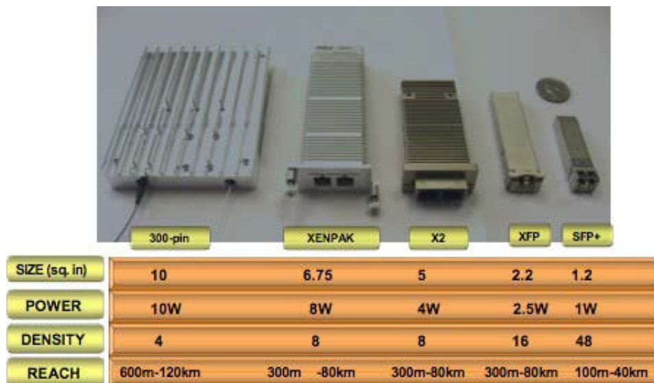
Figure 1: 10G Form Factor comparison. The market trend has always been to reduce to the size and power consumption of the optics and increase the port density on the host board.
