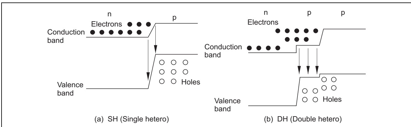
Figure 9 Junction Structure
