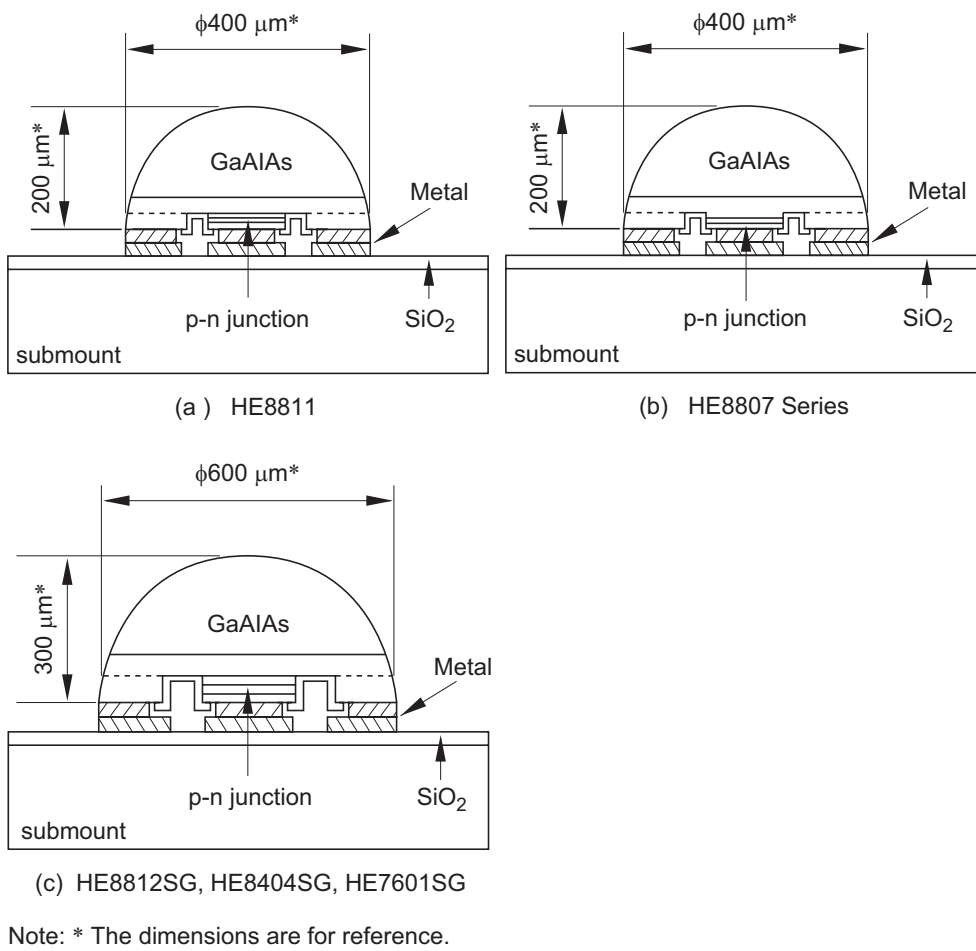
Figure 10 IRED Structures
